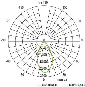
Wide Flood Beam: 54° Beam
