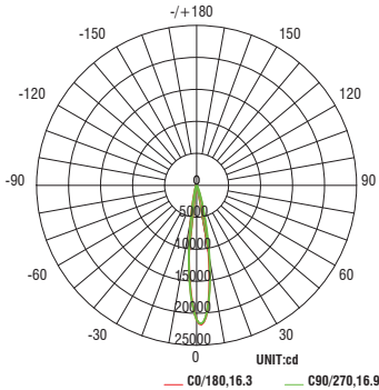
Spot Beam: 17° Beam
