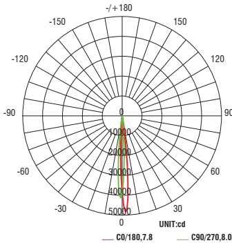
Very Narrow Beam: 7° Beam
