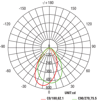
Asymmetric Beam
