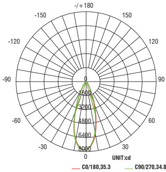
Medium Flood Beam: 36° Beam
