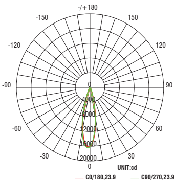
Narrow Flood Beam: 24° Beam
