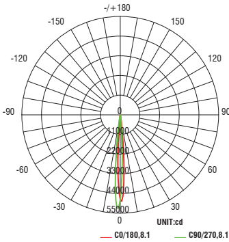
Very Narrow Beam: 8° Beam
