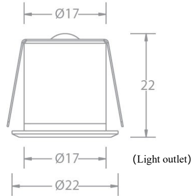
Line Drawing
