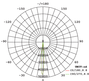
Very Narrow Beam: 8° Beam
