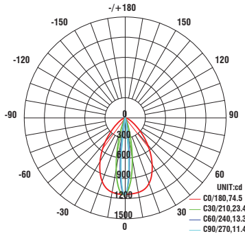
Adjustable Beam - Narrow Flood
