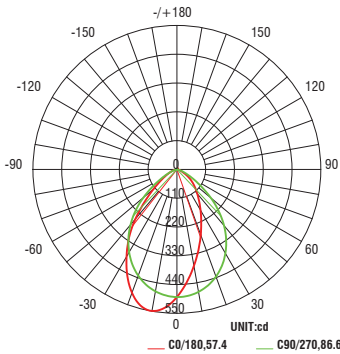
Asymmetric Beam
