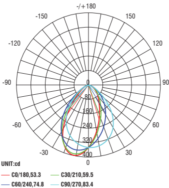
Asymmetric Beam
