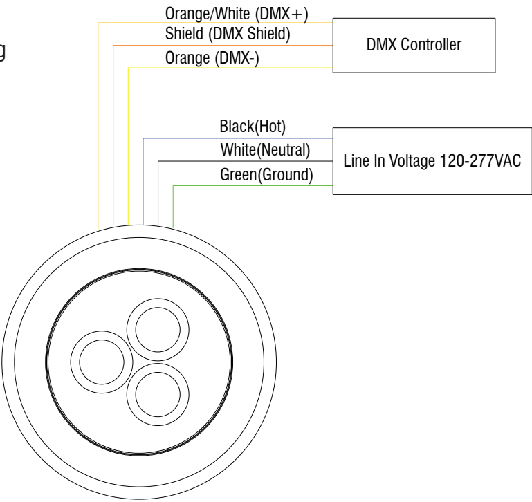
Single Fixture Wiring
