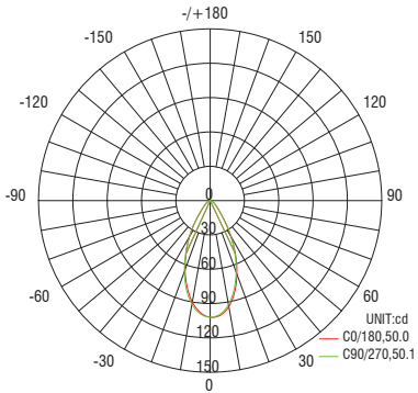
Wide Flood Beam: 50°
