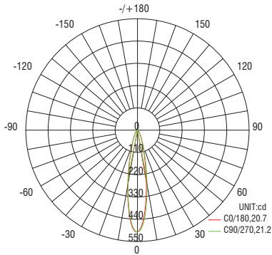
Narrow Flood Beam: 20°
