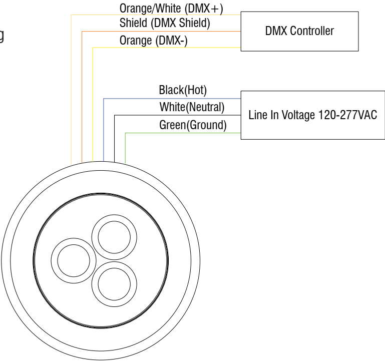
Single Fixture Wiring
