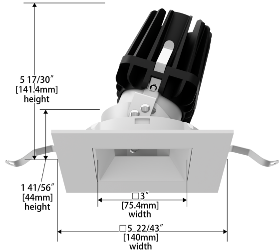
Square Trim (R4FSAT)
