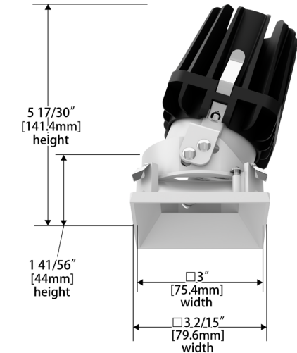
Square Trimless (R4FSAL)
