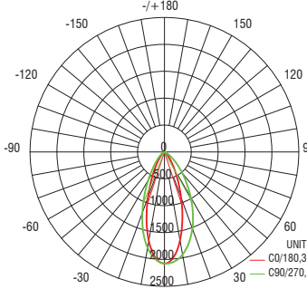
Wall Wash Beam: Asymmetric
